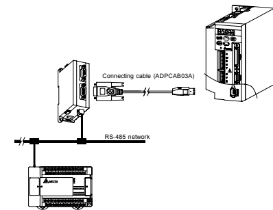
ADP485-01 ⇔ ASD-B (Servo Drive)
