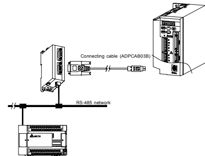
ADP485-01 ⇔ ASD-B (Servo Drive)
